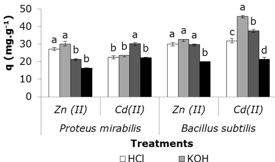
Figure 6. Removal of Zn (II) and Cd (II) from aqueous solution by bacterial biomass subjected to different treatments; 28 \pm 2 °C, metal in solution 1 mM; wet biomass 2 g.L -1 ; stirring at 100 rpm, 24 h. Error bars represent standard deviation of three repetitions per treatment.
