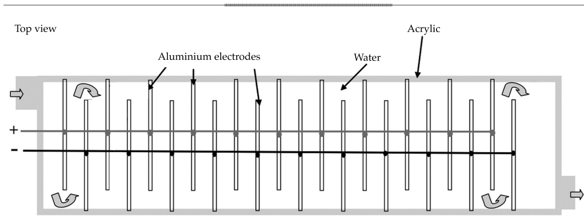
Figure 2. Electrochemical reactor.
